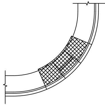
RAMP PAY AREA FOR CURB RAMPS TYPE 2A AND 2B * INCLUDES CONCRETE PEDESTRIAN CURB AS SHOWN
