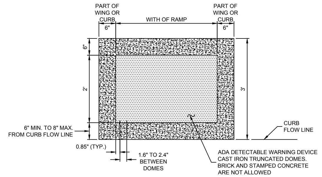
PLAN VIEW OF DETECTABLE WARNING PLATE FOR CURB RAMPS
