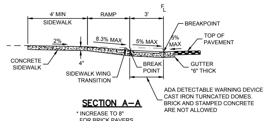
CURB RAMP TYPE 4A SEE NOTE 2
