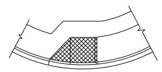
RAMP PAY AREA FOR CURB RAMPS TYPE 4A AND 4B
