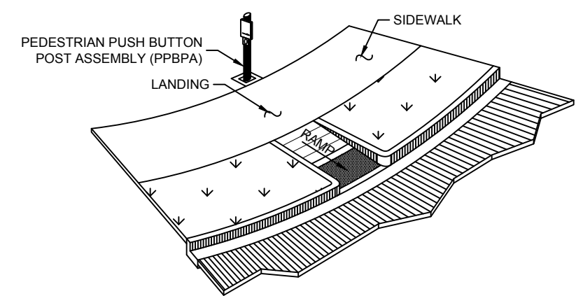
ISOMETRIC VIEW
