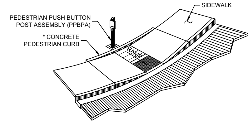
ISOMETRIC VIEW
