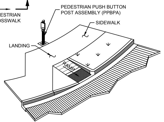
ISOMETRIC VIEW SHOWN WITH PEDESTRIAN PUSH BUTTON POST ASSEMBLY (PPBPA)
