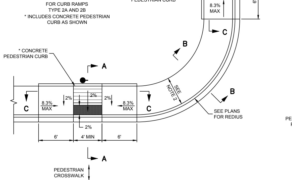
RAMP PAY AREA FOR CURB RAMPS TYPE 2A AND 2B * INCLUDES CONCRETE PEDESTRIAN CURB AS SHOWN
