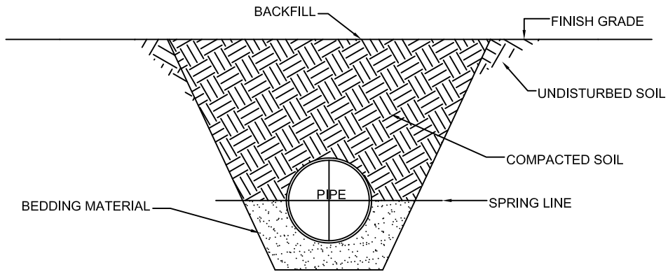
REINFORCED CONCRETE PIPE
