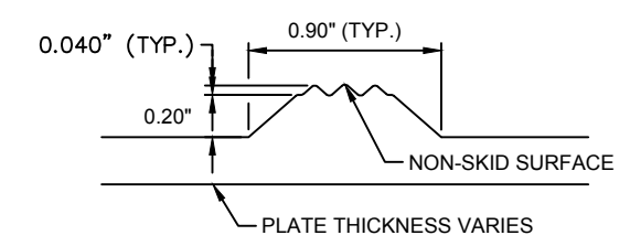
ELEVATION VIEW OF DETECTABLE WARNING PLATE FOR CURB RAMPS
