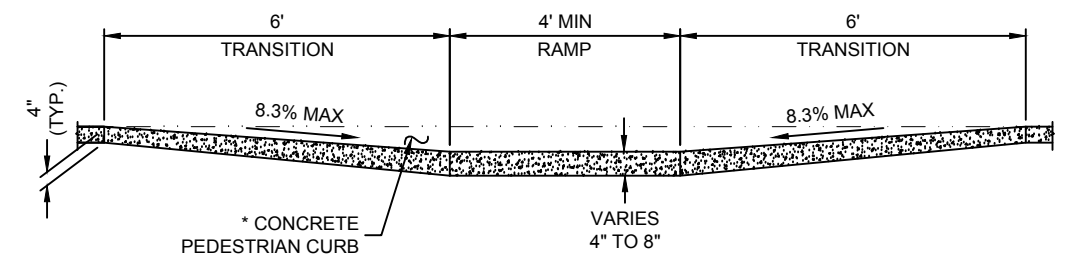
SECTION C-C
