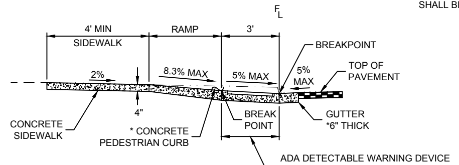
SECTION F-F
