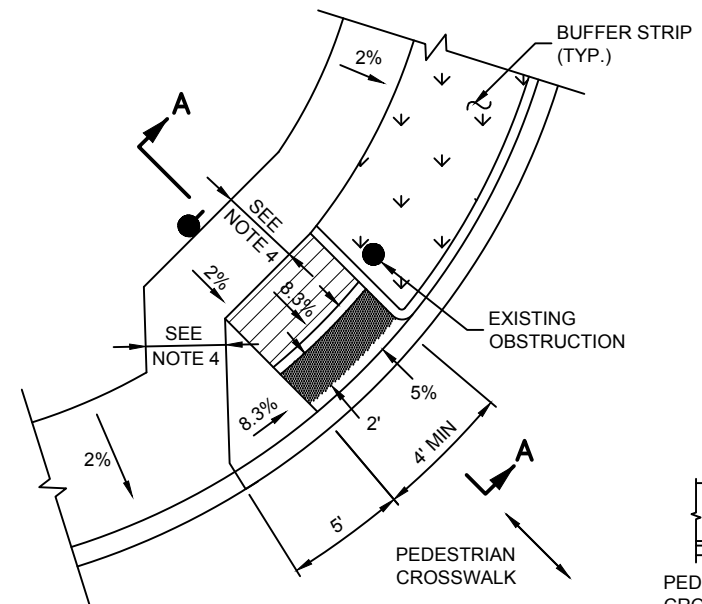
CURB RAMP TYPE 4A SEE NOTE 2
