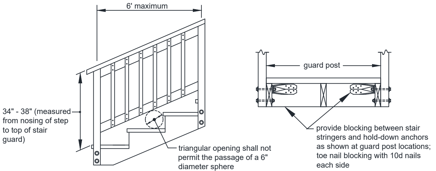
FIGURE 40: STAIR GUARD
