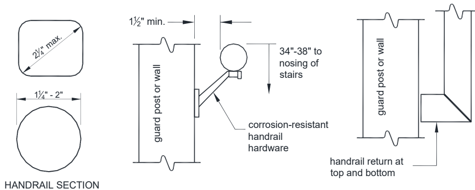
FIGURE 41: HANDRAILS
