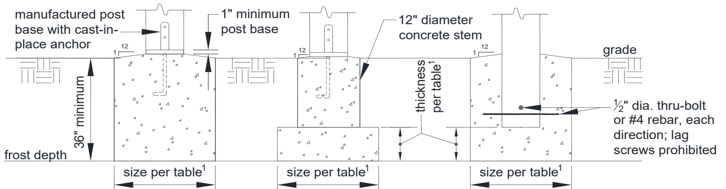
FIGURE 15: FOOTINGS
