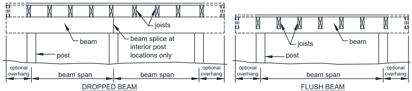
FIGURE 12: BEAM TYPES
