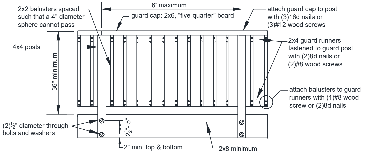
FIGURE 32: GUARD CONSTRUCTION
