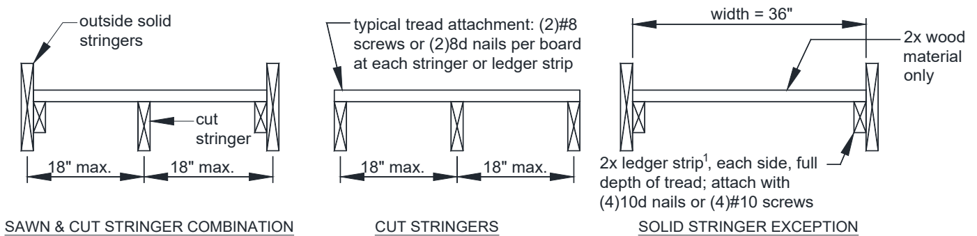
FIGURE 39: STRINGER TREADS
