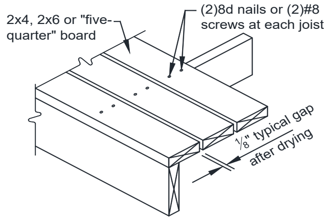
FIGURE 1: TYPICAL DECKING
