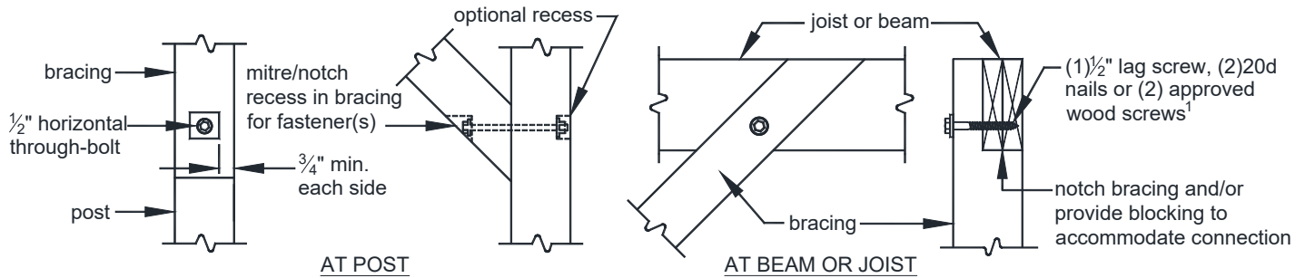
FIGURE 30: TYPICAL CONNECTIONS OF 6x6 KNEE-BRACING
