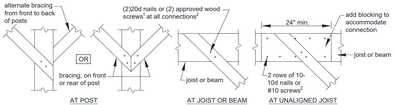
FIGURE 29: TYPICAL CONNECTIONS OF 2x KNEE-BRACING
