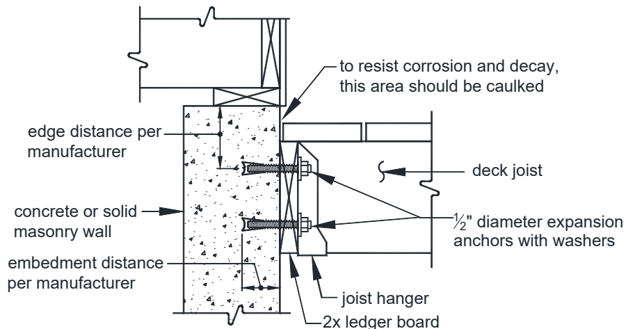
FIGURE 20: LEDGER BOARD-TO-SOLID FOUNDATION ATTACHMENT
