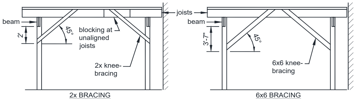
FIGURE 28: METHOD 3 - KNEE-BRACING AT JOIST-POST LOCATIONS
