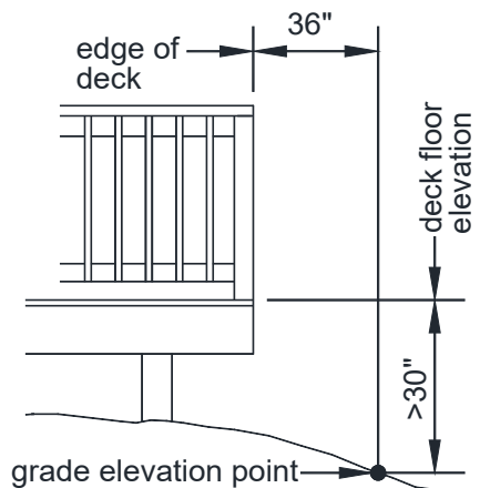
FIGURE 31: WHEN A GUARD IS REQUIRED
