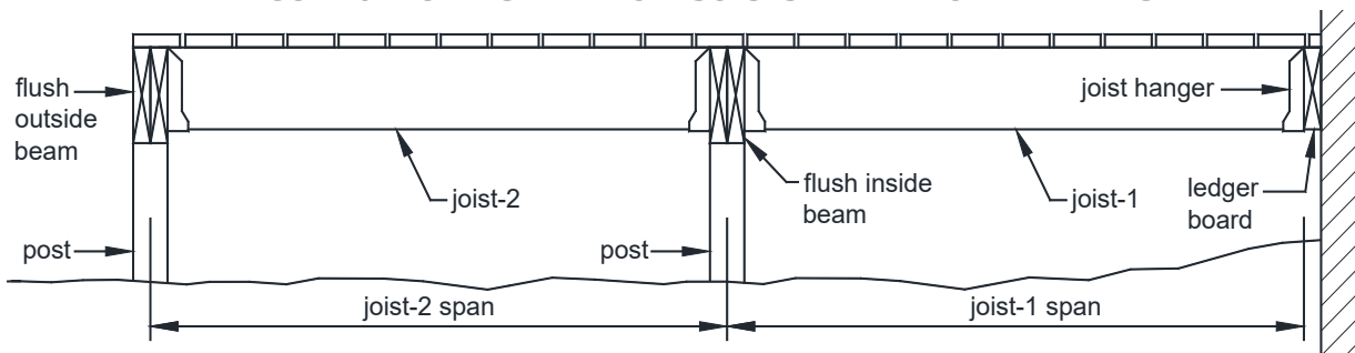
FIGURE 7: MULTI-SPAN DECK - JOISTS WITH FLUSH BEAMS
