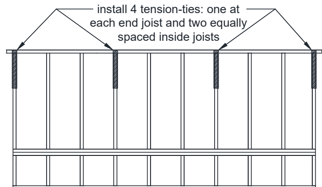
FIGURE 25: METHOD 1 - TENSION TIE LOCATIONS
