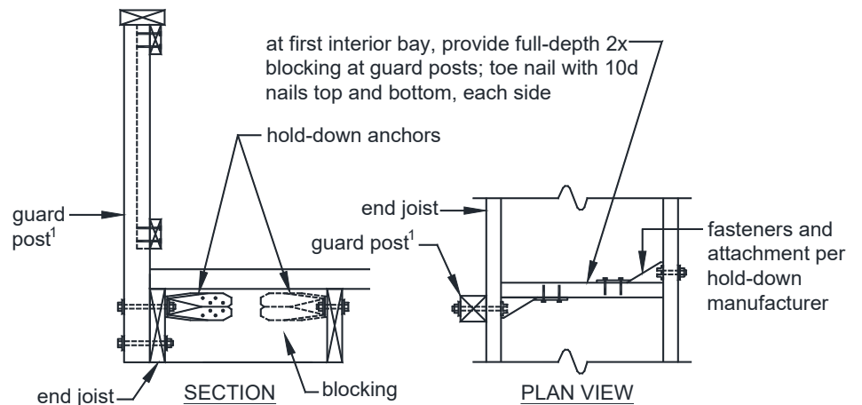
FIGURE 34: GUARD POST-TO-END JOIST
