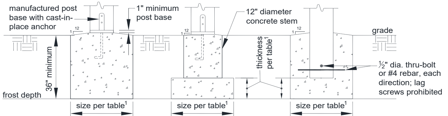
FIGURE 15: FOOTINGS
