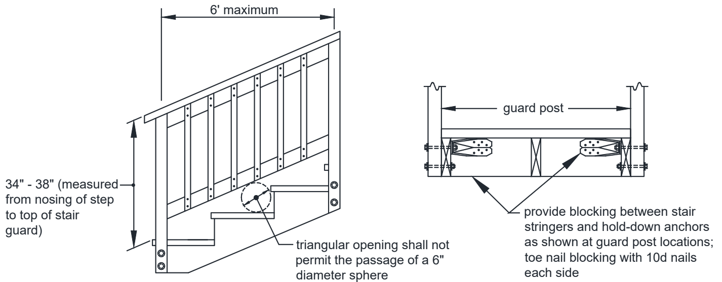
FIGURE 40: STAIR GUARD
