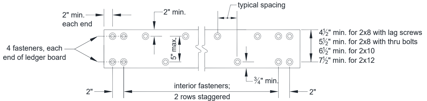
FIGURE 23: LEDGER BOARD FASTENER SPACING AND CLEARANCES
