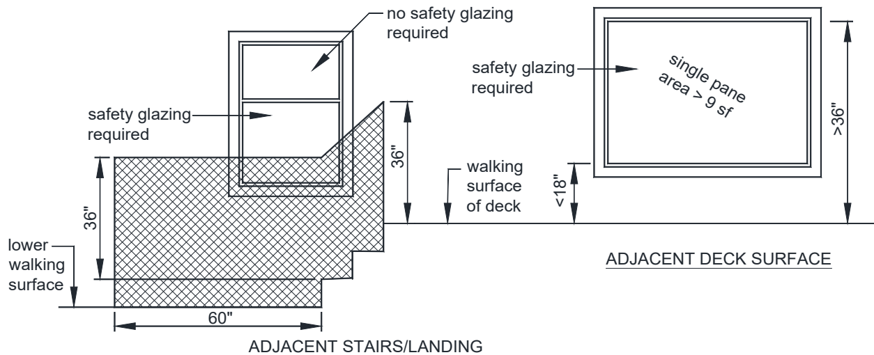
FIGURE 3: SAFETY GLAZING REQUIREMENTS
