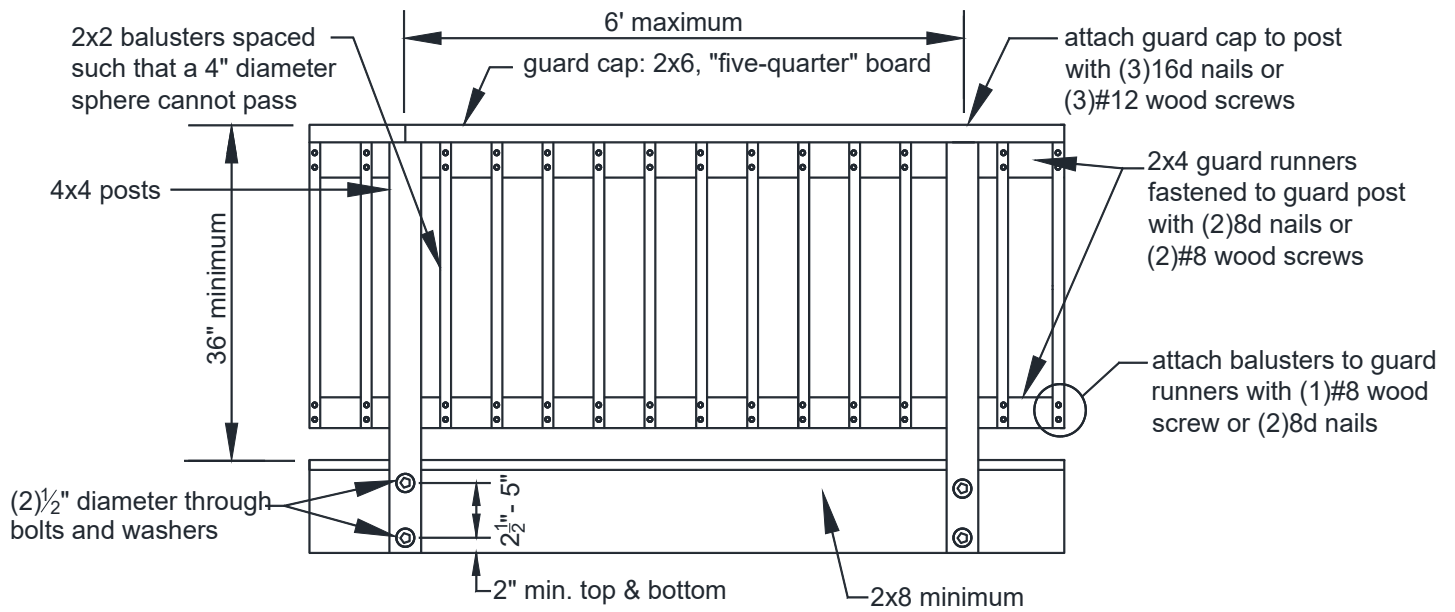
FIGURE 32: GUARD CONSTRUCTION
