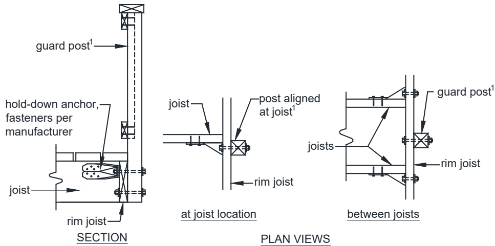
FIGURE 35: GUARD POST-TO-RIM JOIST
