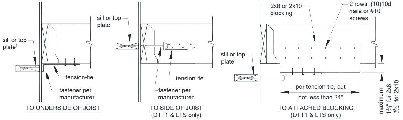
FIGURE 26: METHOD 1 - TENSION-TIE CONNECTION
