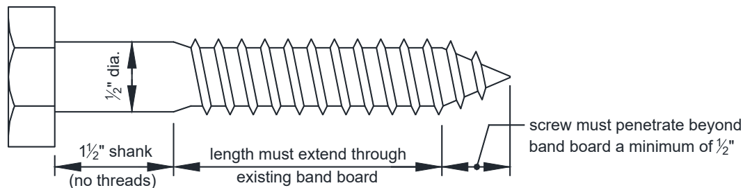
FIGURE 24: LAG SCREW
