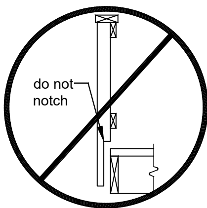
FIGURE 33: POST NOTCHES PROHIBITED
