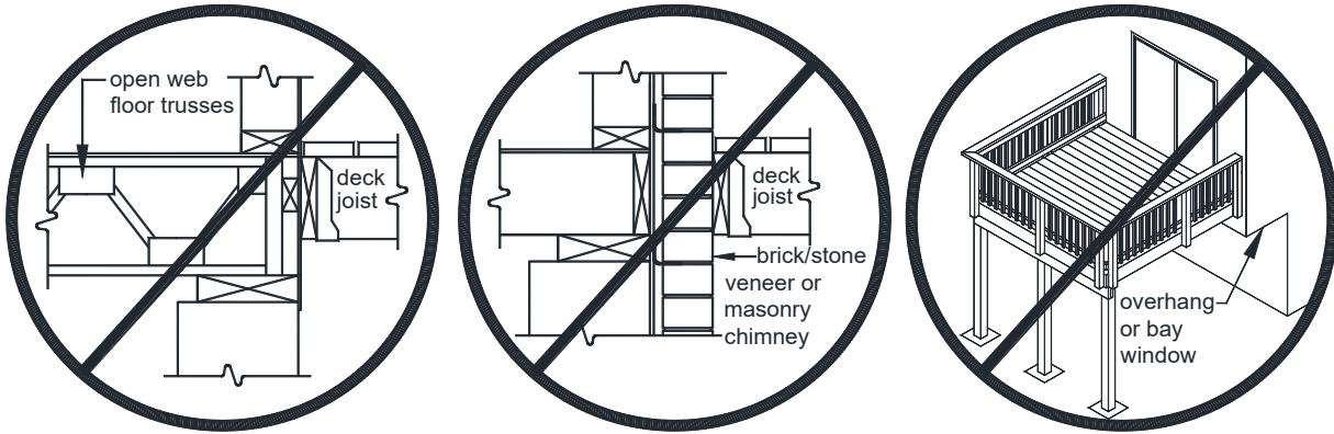
FIGURE 22: PROHIBITED LEDGER ATTACHMENTS
