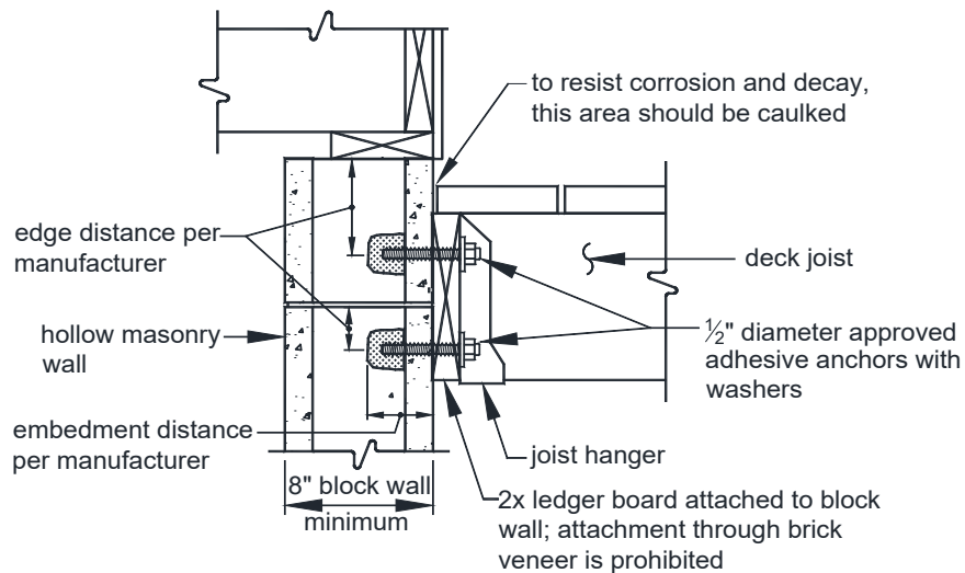
FIGURE 21: LEDGER BOARD-TO-HOLLOW FOUNDATION ATTACHMENT
