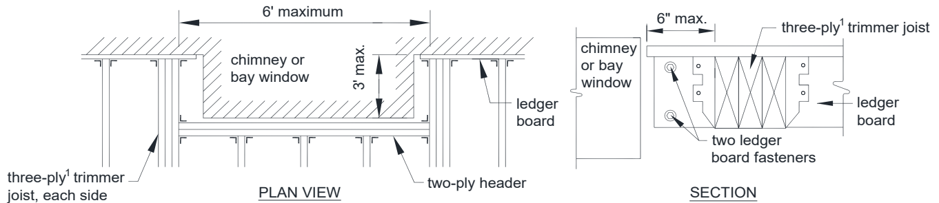
FIGURE 9: FRAMING AT CHIMNEY OR BAY WINDOW
