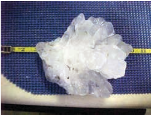
The Aurora, Nebraska record hailstone
